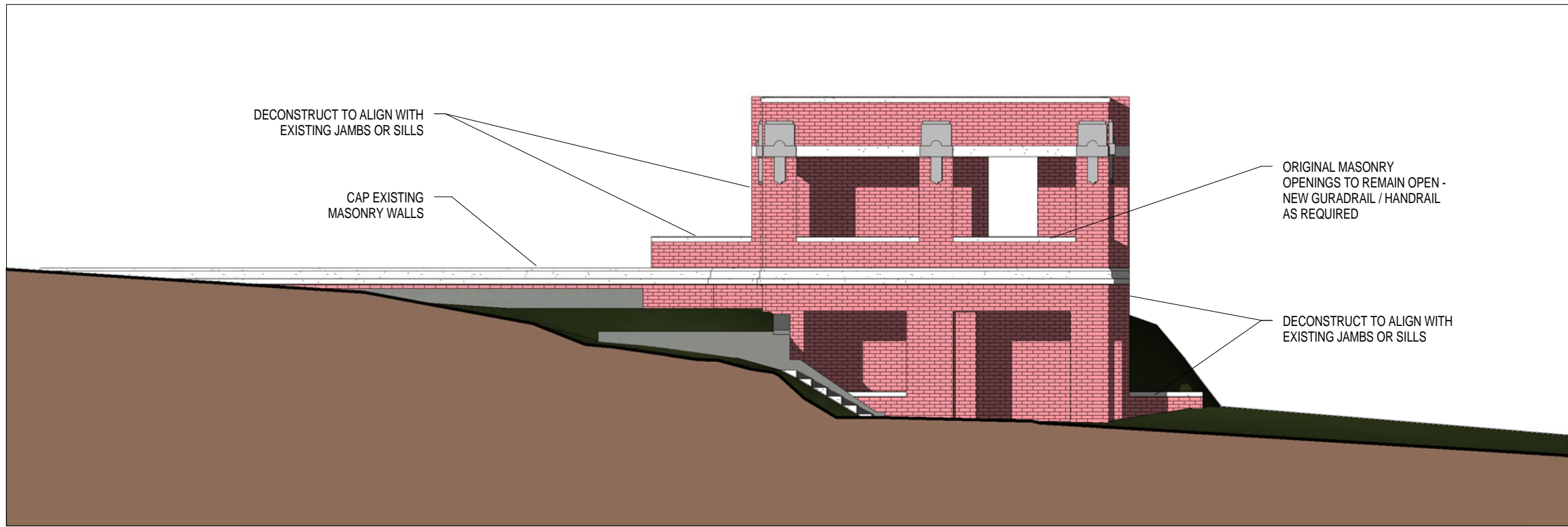
WEST ELEVATION
